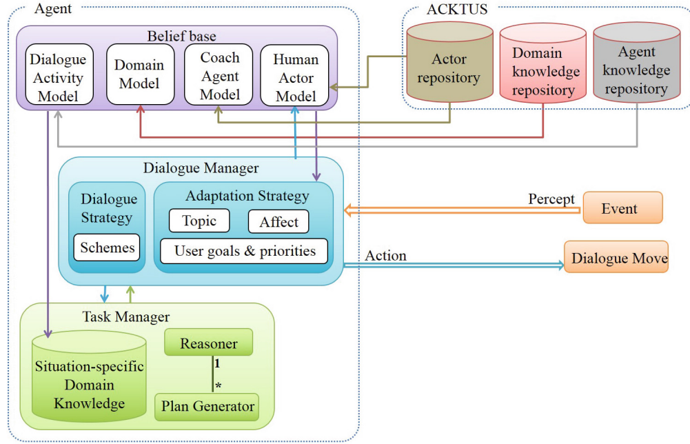
Fig. 2. Architecture of the human-agent dialogue system.
